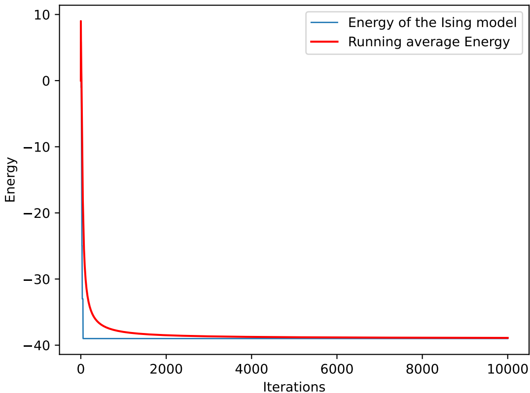
Evolution of a stochastic simulation of the 1D Ising model, at \beta = 2 J = 1 h = 1
